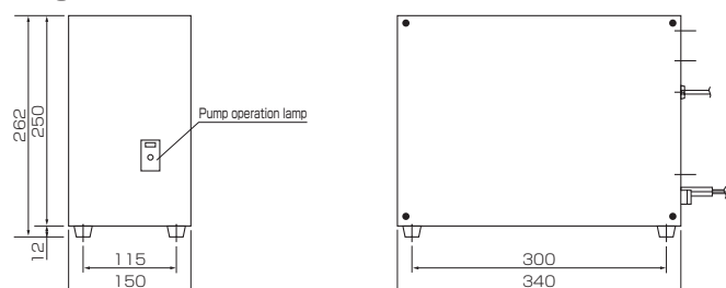
Cooling unit
